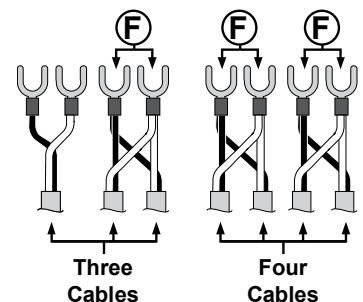
'Ezi connect' cable connector for water heater models: INFINITY 32, 26i, ENVIRO & HD/HDC Series
